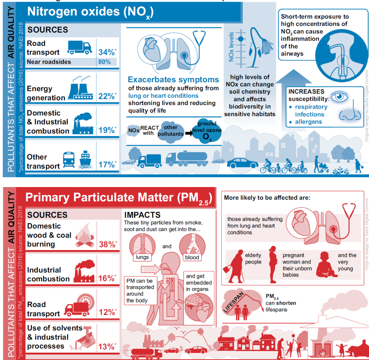
Figure 6. Air pollutants, sources and potential health impacts of NO x and PM 2.5 from the Clean Air Strategy 2019 12
