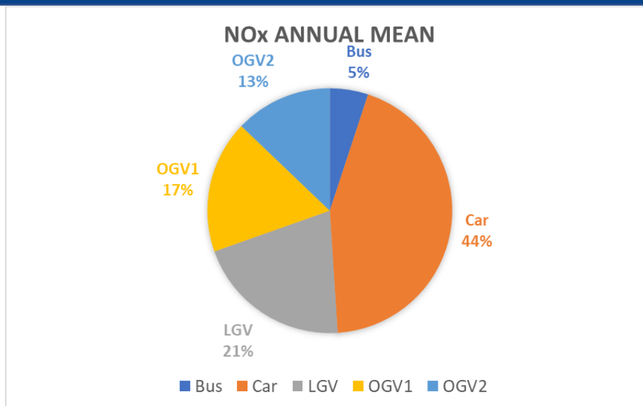
Figure 8. NOx Source Apportionment at St Paul’s Street (AQMA 4)
